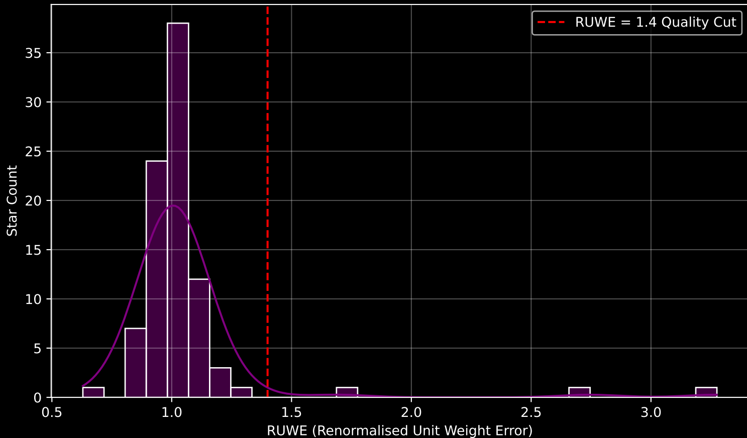
GAPOGEE DR17 Field [013+00] RUWE Distribution (n= 89)
