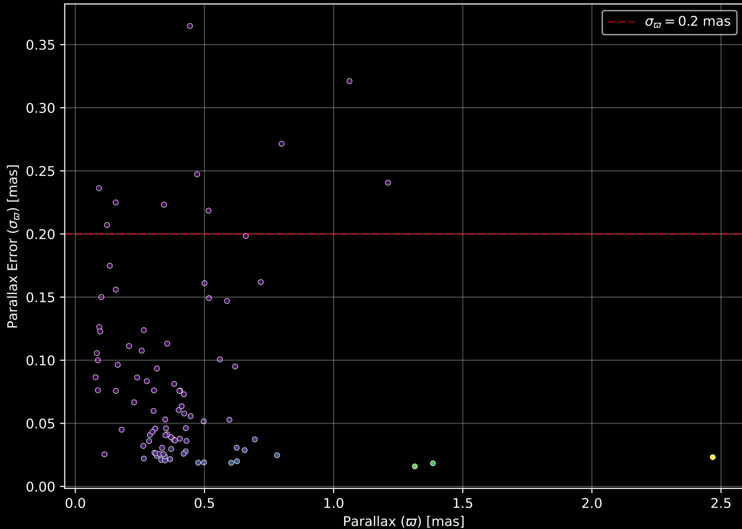
APOGEE DR17 Field: [013+00] Parallax Quality (n= 90)
