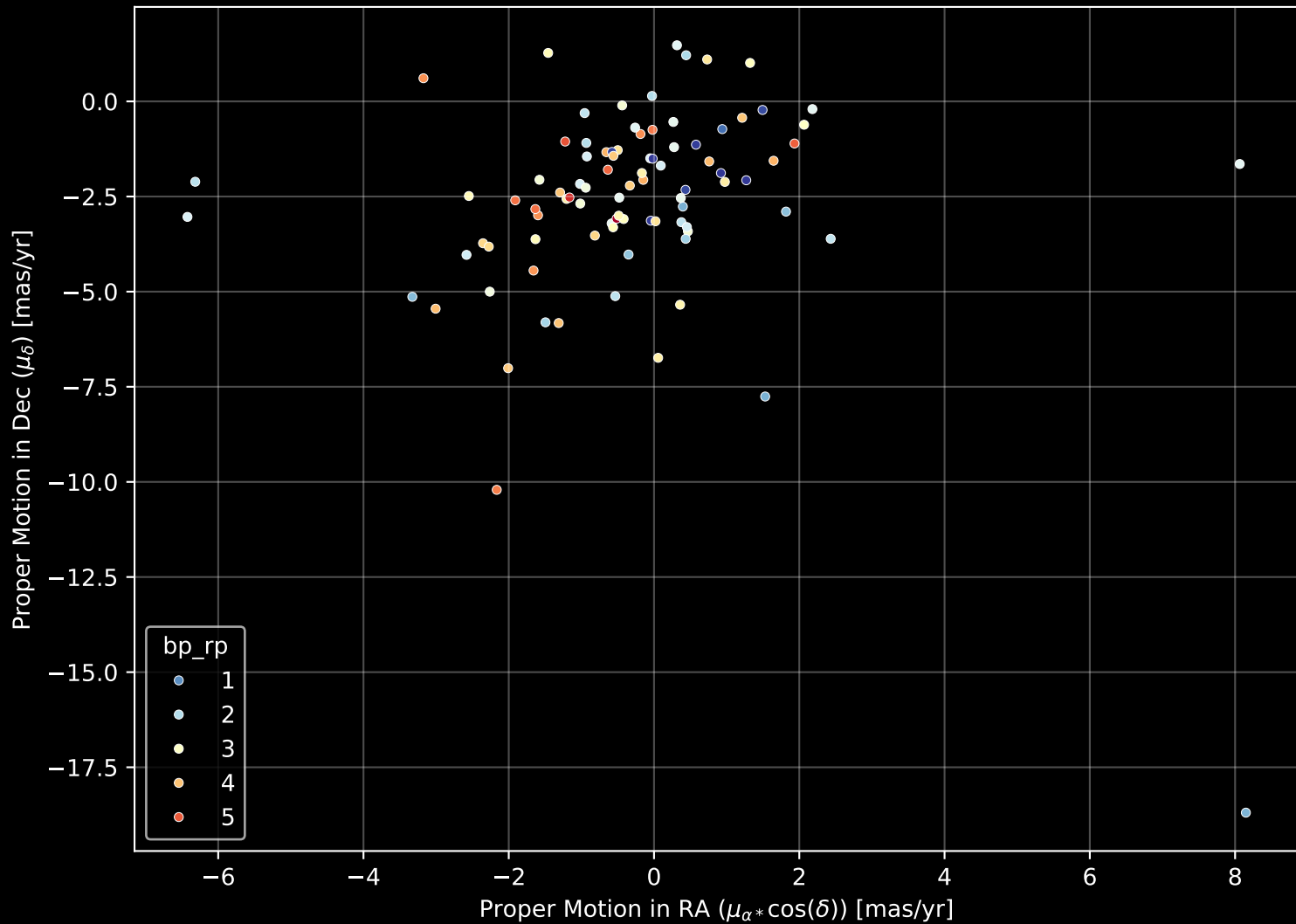
APOGEE DR17 Field: [013+00] Proper Motion Diagram (n= 90)
