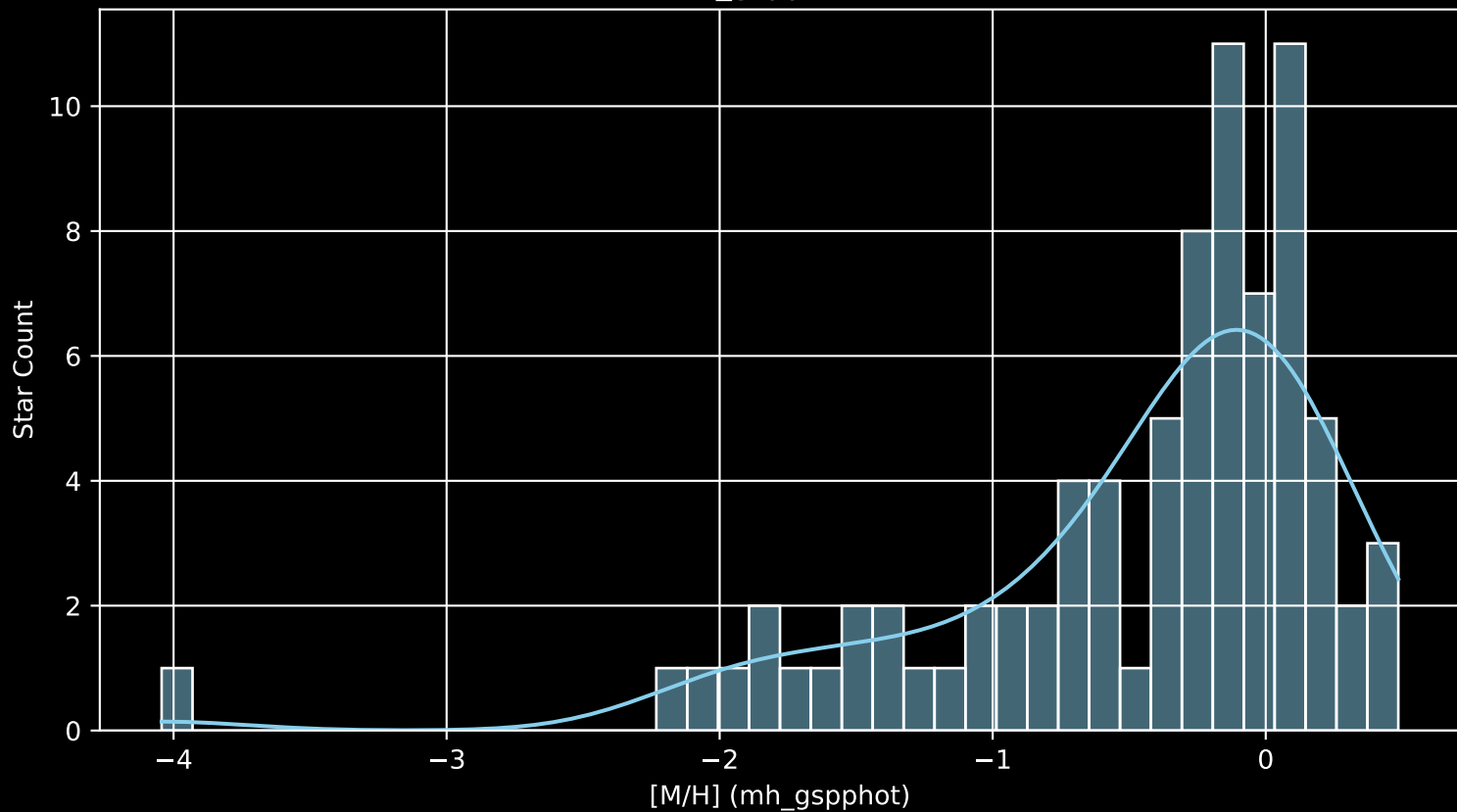
APOGEE DR17 Field: [013+00 [M/H] (mh_gspphot) (n= 81)
