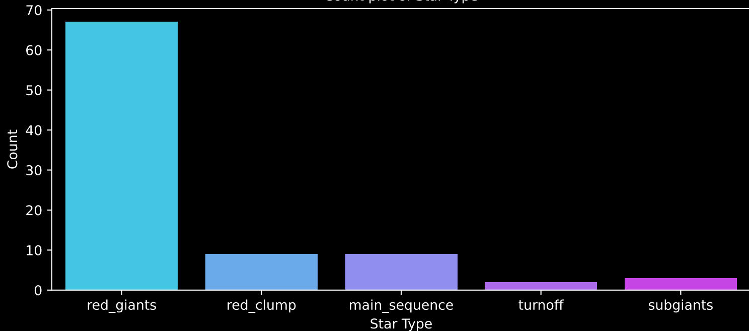
APOGEE DR17 Field: [013+00] Count plot of Star Type
